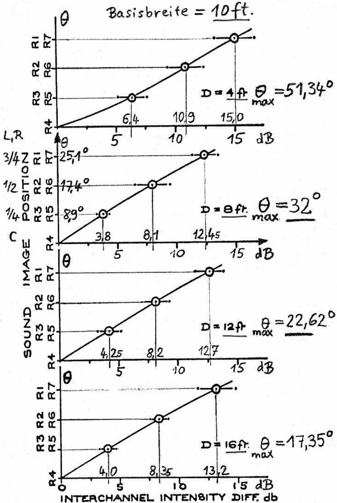
Fig. 5. Effect of variation of listening distance. \pm 51,3^\circ , \pm 32^\circ , \pm 22,6^\circ and 17,4^\circ . Central listening positions. 6 subjects tested. Half-curves only plotted.
